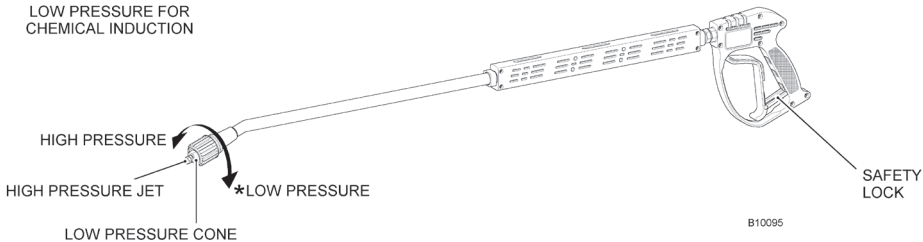
FIXED SINGLE LANCE WITH ADJUSTABLE NOZZLE
